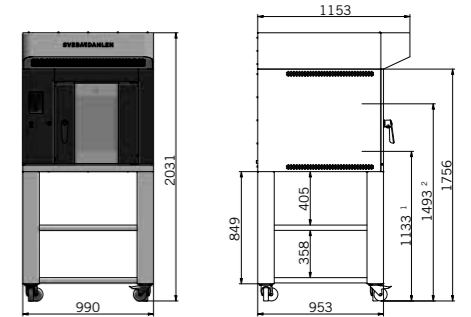
Dimensional sketch SR120 with extra storage shelf.
